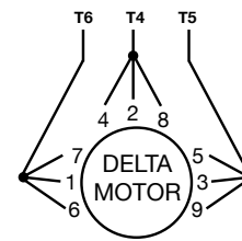
9 LEAD, 230V LOW VOLTAGE, MOTOR CONNECTIONS
