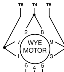
9 LEAD, 230V LOW VOLTAGE, MOTOR CONNECTIONS
