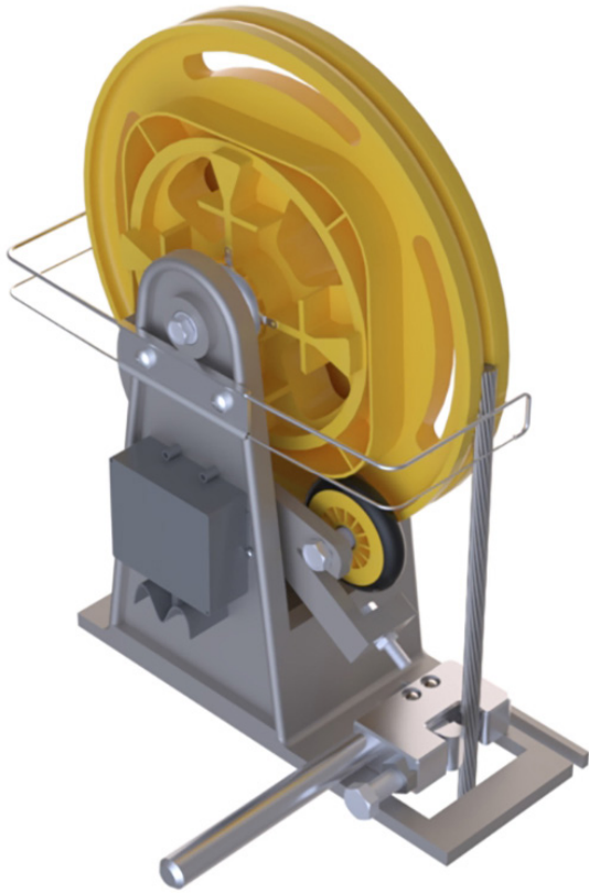
90-10057468 Governor Rope Clamp
