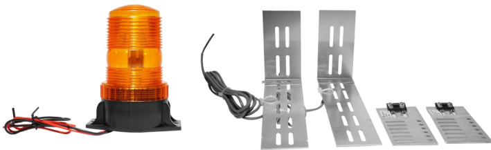
Part No. DLMS1-D Elevator Cab Door Monitoring System
