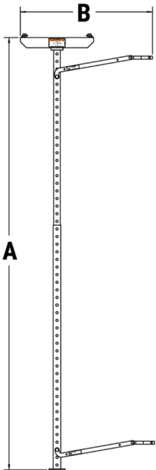
Omega / Hat Rail Configuration
