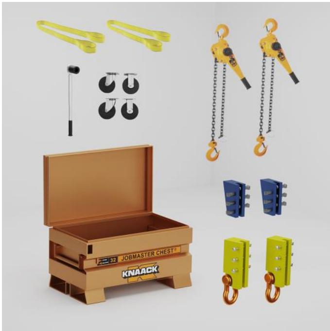
Part No. RGK-06T 6-Ton Car Hanging Kit
