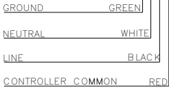
POWER CABLE WIRING
