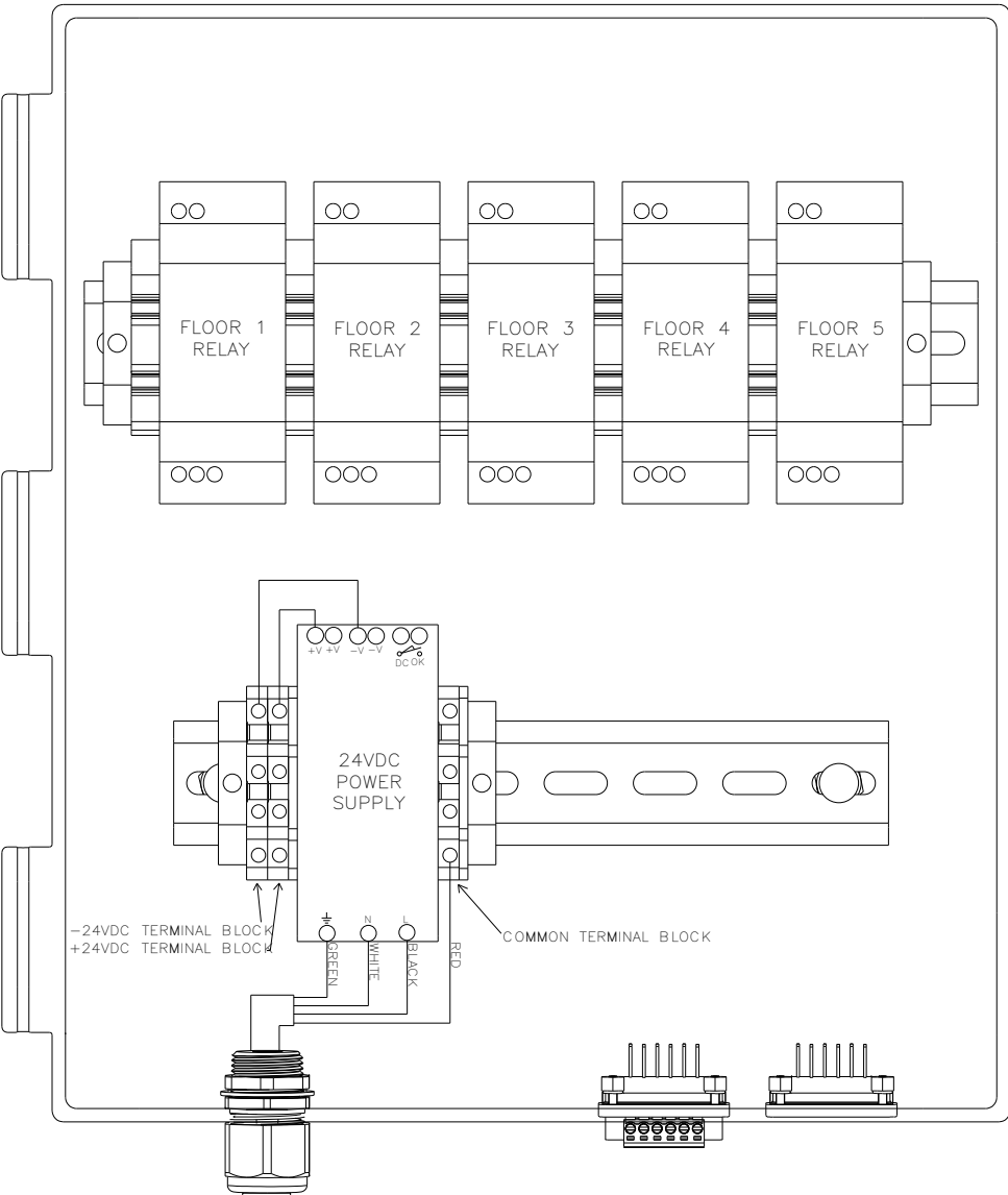
ENCLOSURE TOP VIEW
