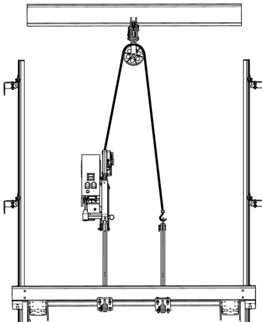
2:1 Installation
