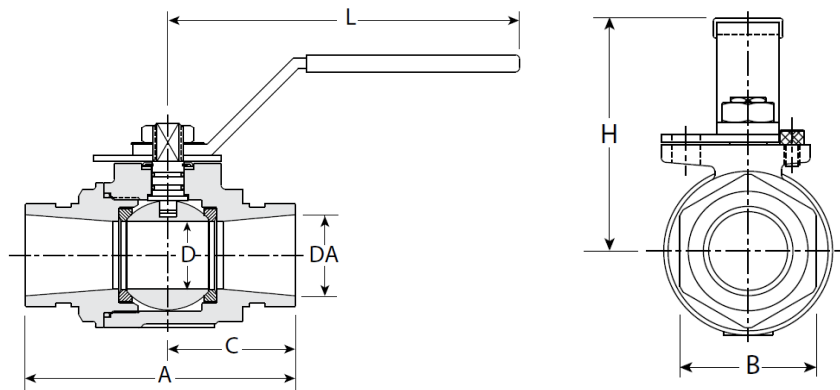
Dimensions Series 726 1-1/2" to 3"
