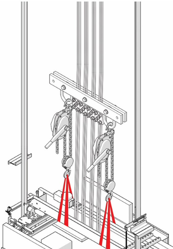
Lifting Bar in Context
