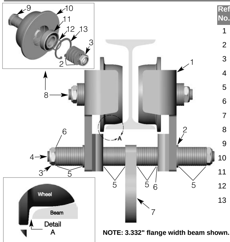
Figure 1 - CT-A Series Complete Plain Trolley
