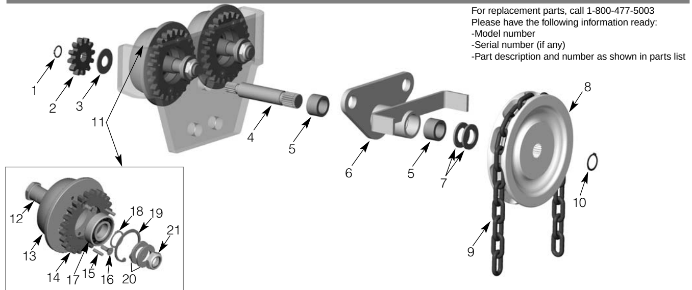
Figure 2 - CT-A Series Geared Trolley
