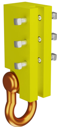
11-190-M Rail Block w/ Clevis, 5/8"
