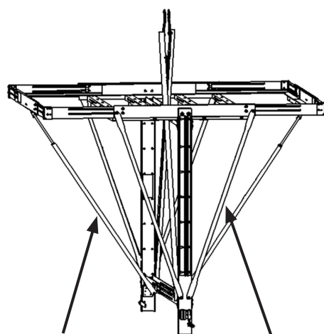
11-305-SK Support Kit
